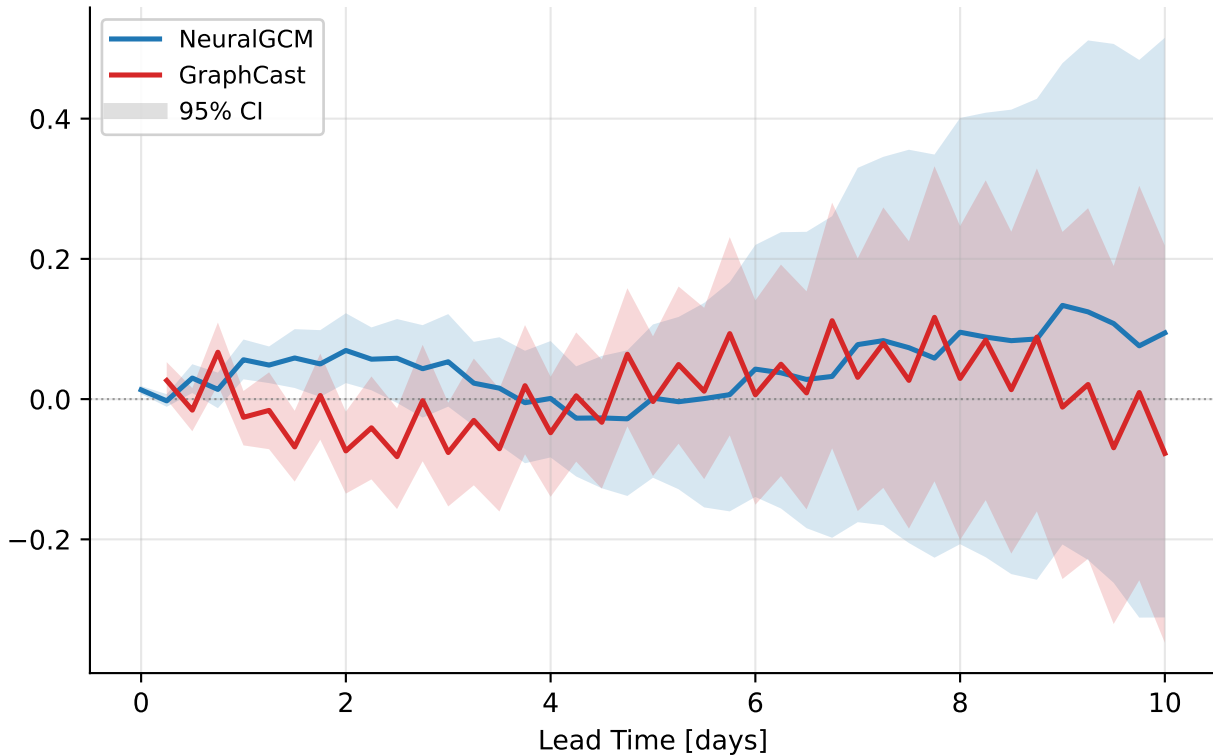
Europe heat-wave 2023-07-05..2023-09-01 — footprint temperature@850 hPa (mean of 69 rollouts)
