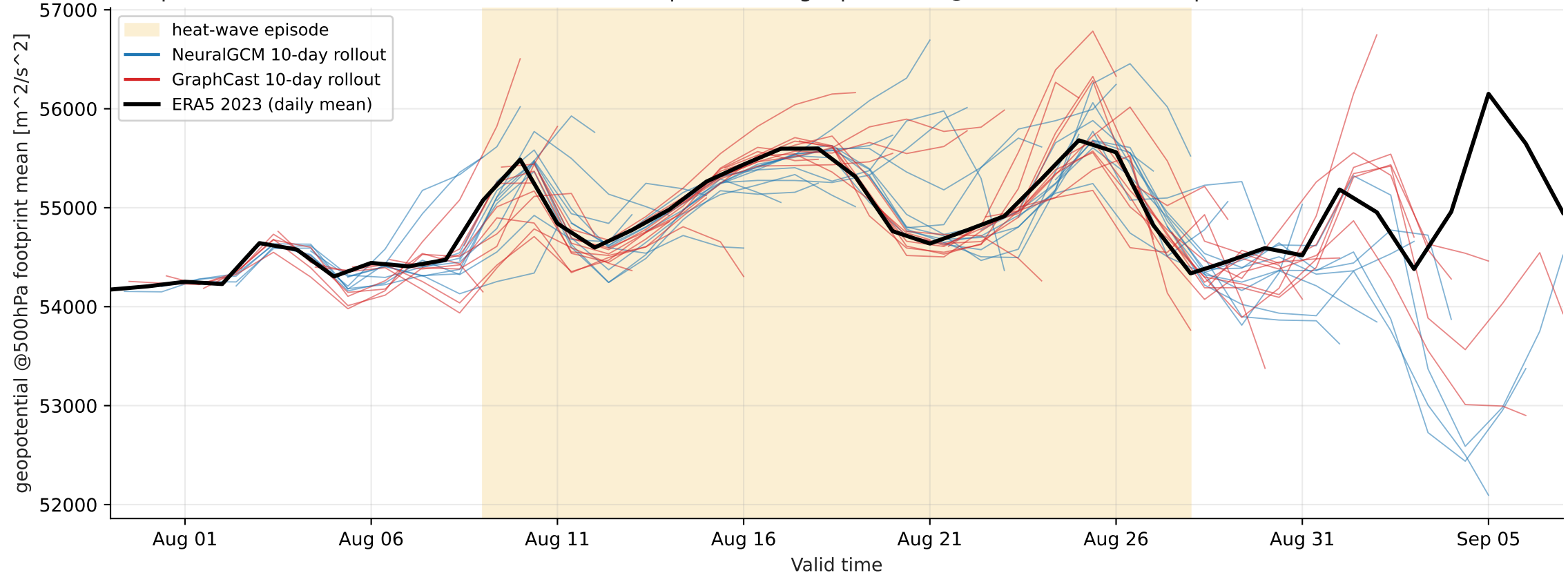
Europe heat-wave 2023-08-09..2023-08-28 — footprint-mean geopotential @ 500 hPa (cordex, > p99)
