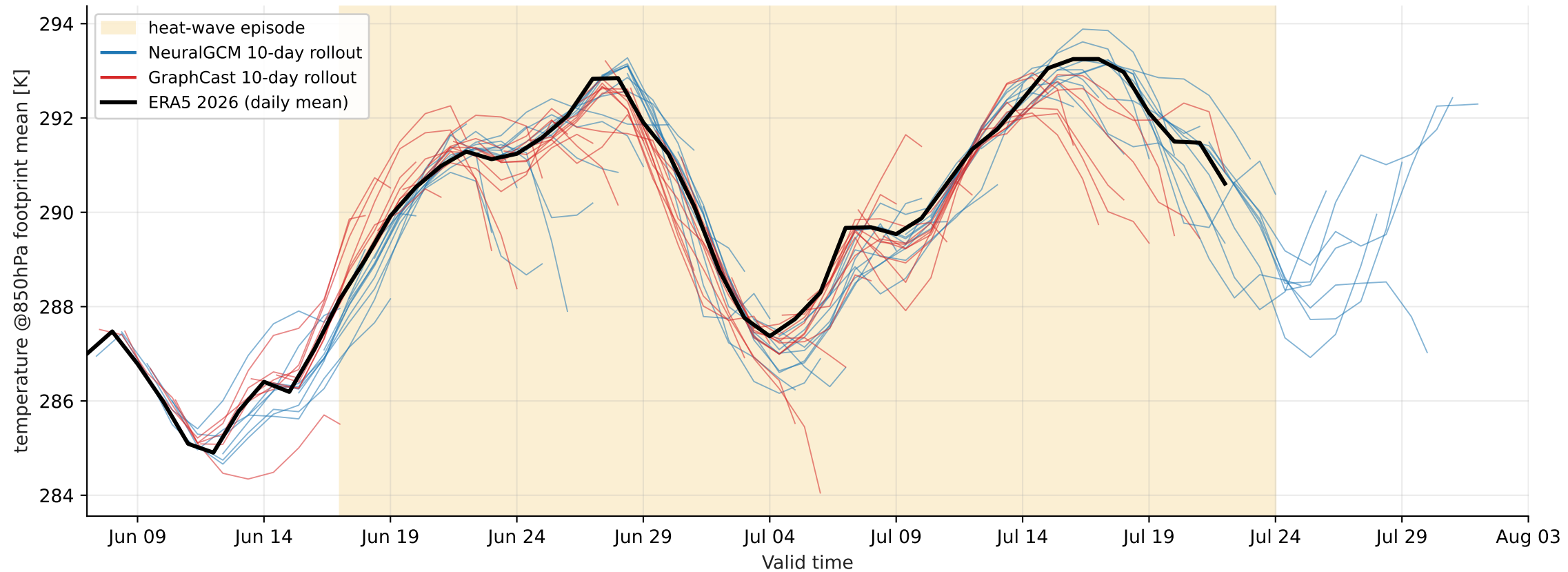
Europe heat-wave 2026-06-17..2026-07-24 — footprint-mean temperature @ 850 hPa (cordex, > p99)
