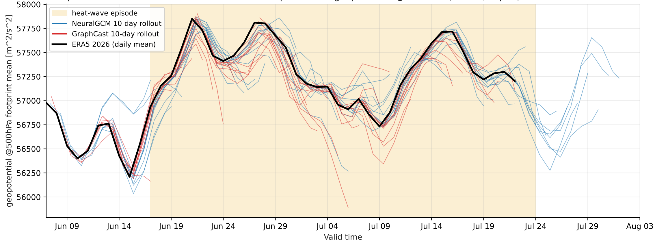
Europe heat-wave 2026-06-17..2026-07-24 — footprint-mean geopotential @ 500 hPa (cordex, > p99)
