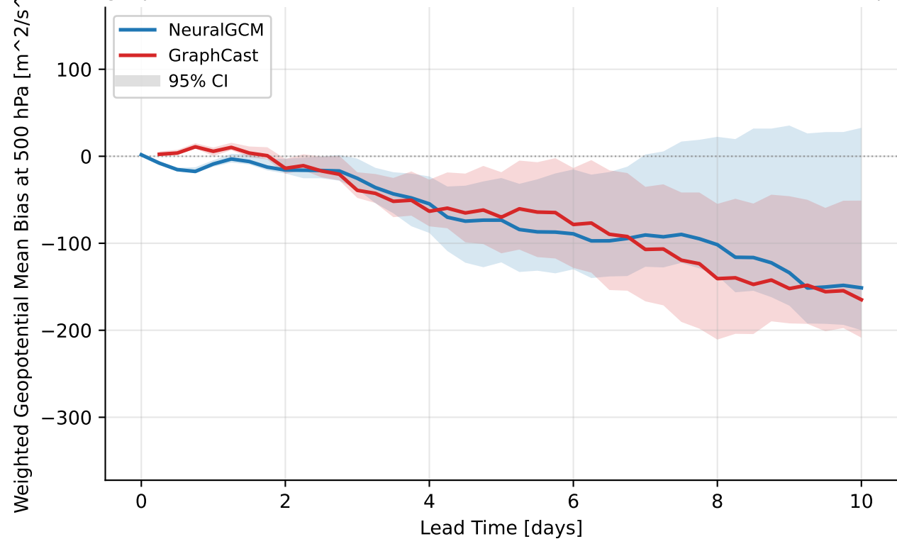
geopotential@500 hPa — mean bias over all cordex heat waves (9 events, > p99)
