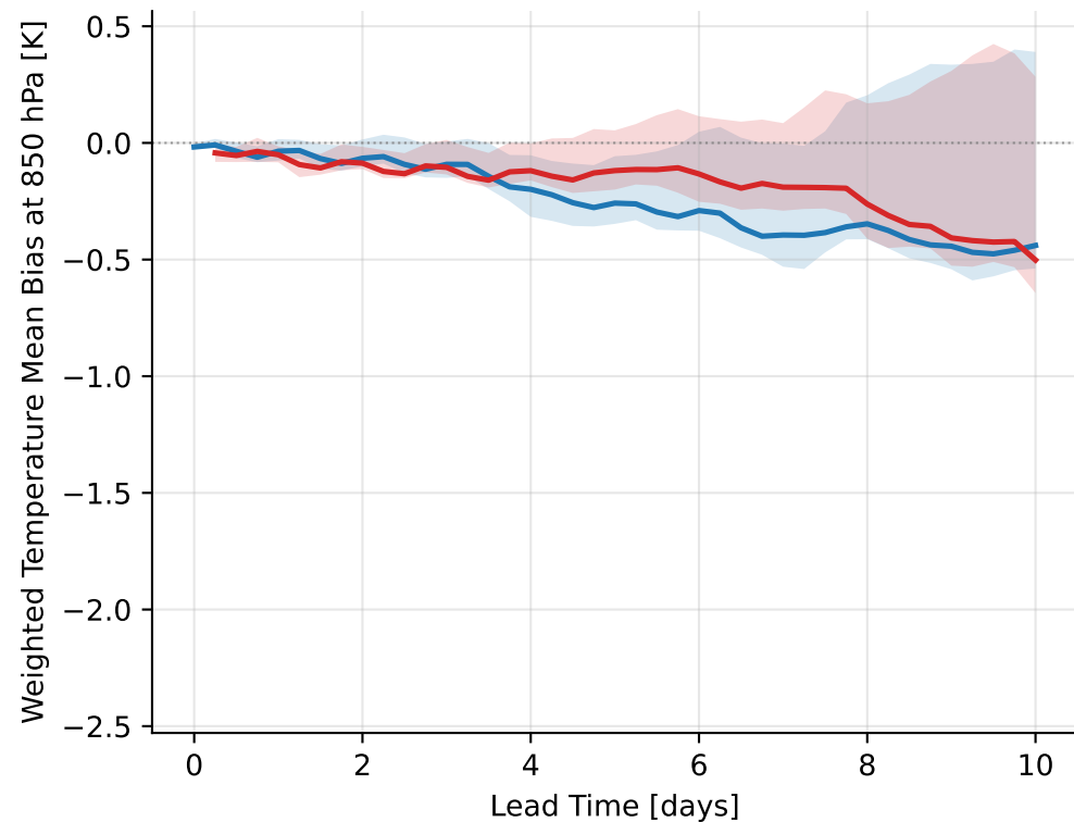
temperature@850 hPa — mean bias over cordex heat waves per year (> p99)
