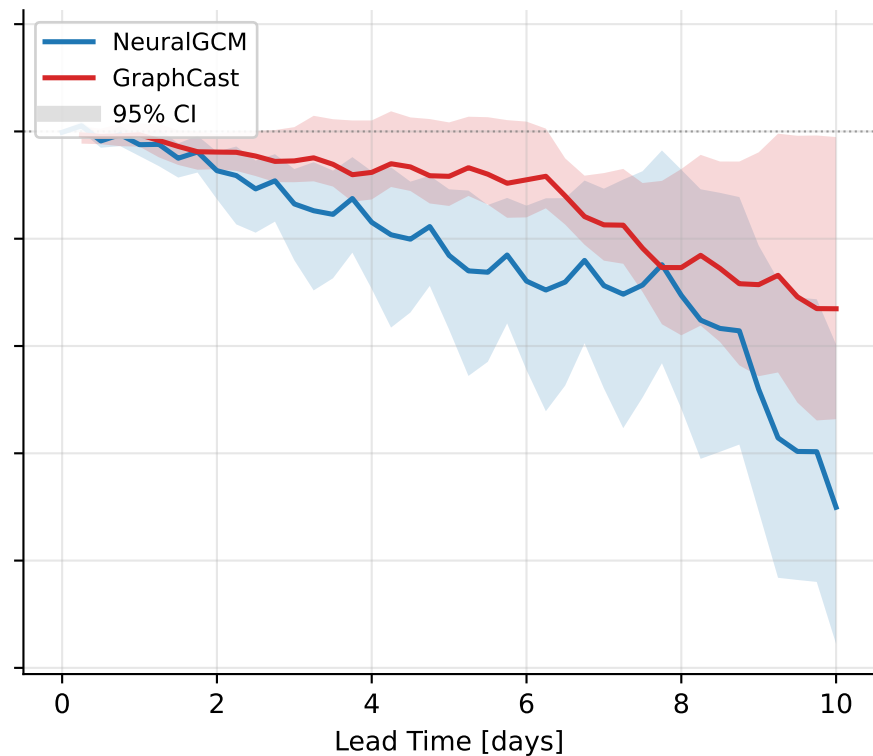
temperature@850 hPa — mean bias over cordex heat waves per year (> p99)
