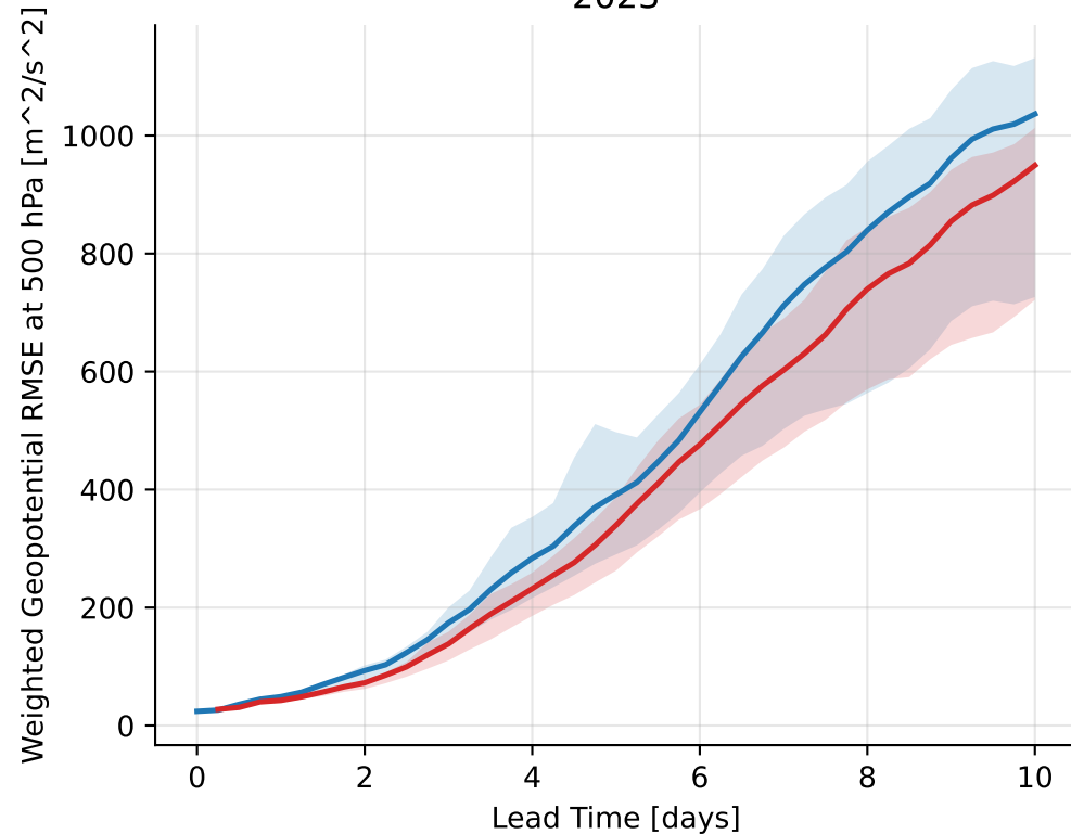
geopotential@500 hPa — mean RMSE over cordex heat waves per year (> p99)
