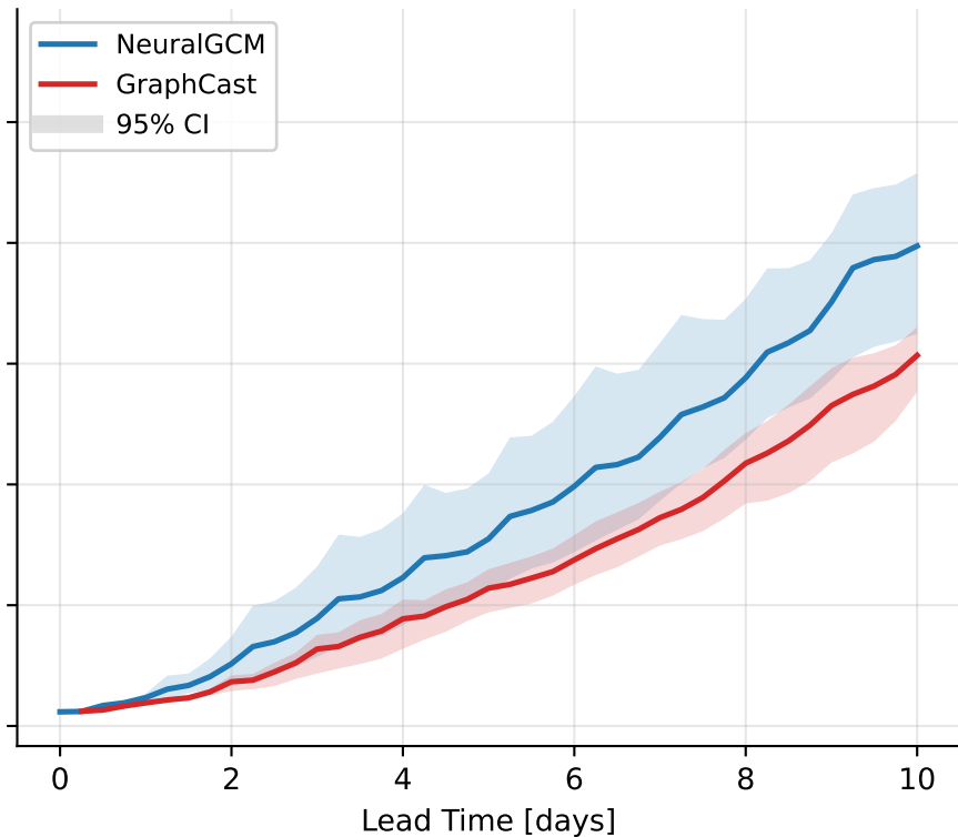
geopotential@500 hPa — mean RMSE over cordex heat waves per year (> p99)
