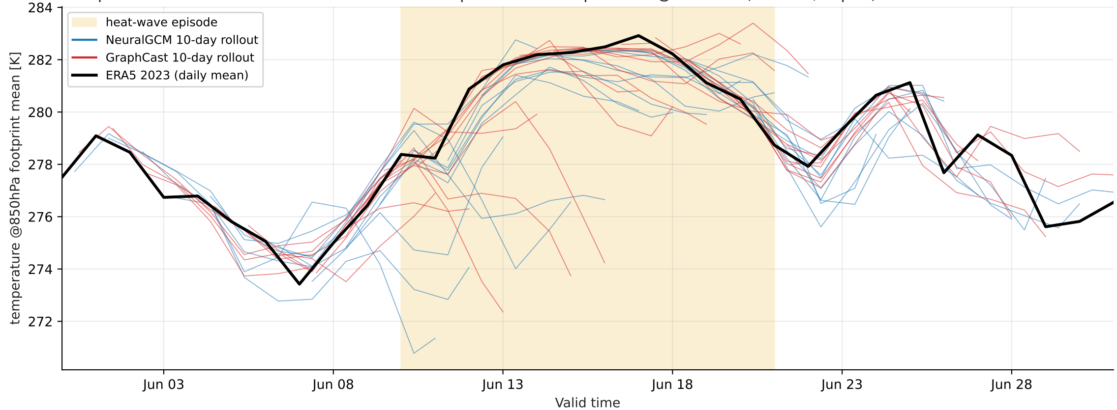
Europe heat-wave 2023-06-10..2023-06-21 — footprint-mean temperature @ 850 hPa (mixture, > p99)
