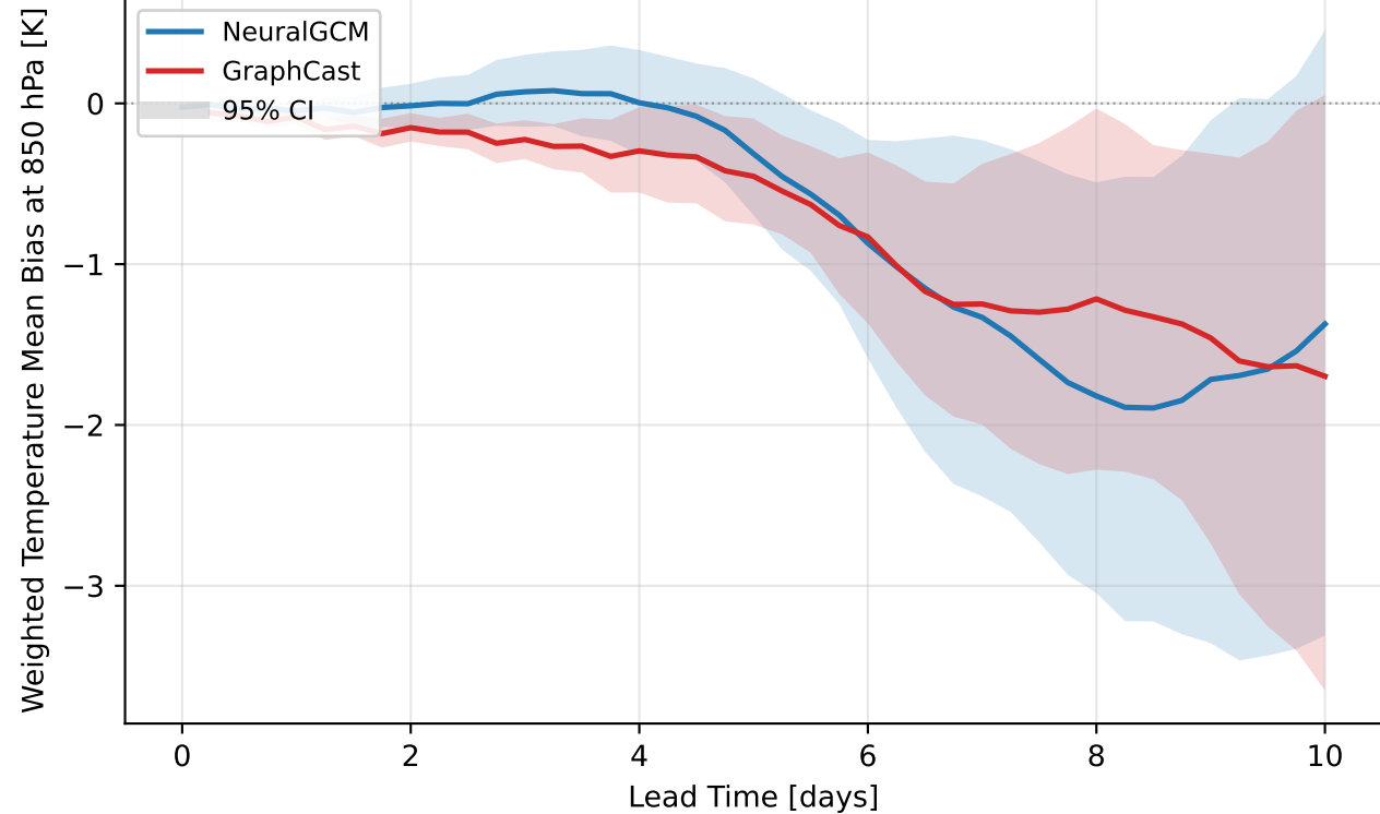
Europe heat-wave 2023-09-29..2023-10-11 — footprint temperature@850 hPa (mean of 23 rollouts)
