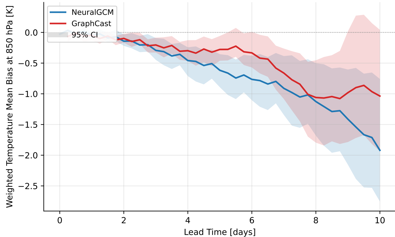
temperature@850 hPa — mean bias over the 6 2026 mixture heat waves (6 events, > p99)
