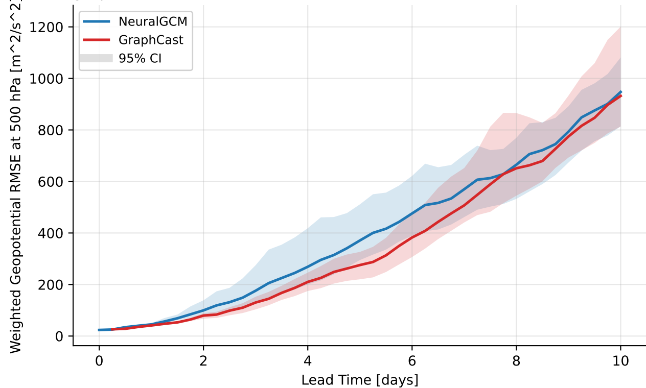
geopotential@500 hPa — mean RMSE over the 6 2026 mixture heat waves (6 events, > p99)
