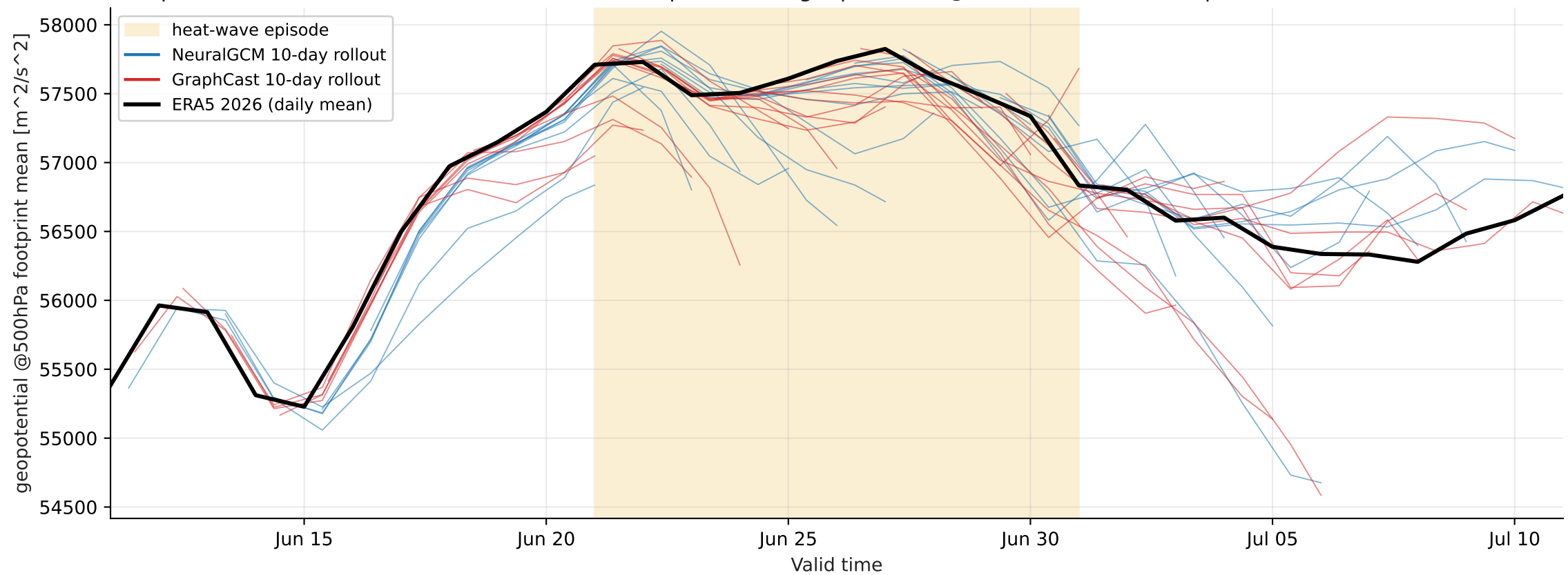
Europe heat-wave 2026-06-21..2026-07-01 — footprint-mean geopotential @ 500 hPa (mixture, > p99)
