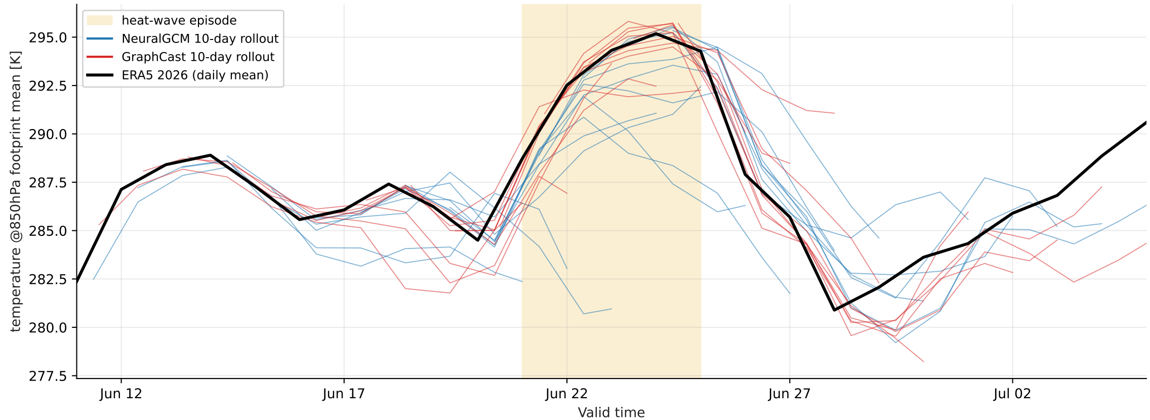
Europe heat-wave 2026-06-21..2026-06-25 — footprint-mean temperature @ 850 hPa (mixture, > p99)
