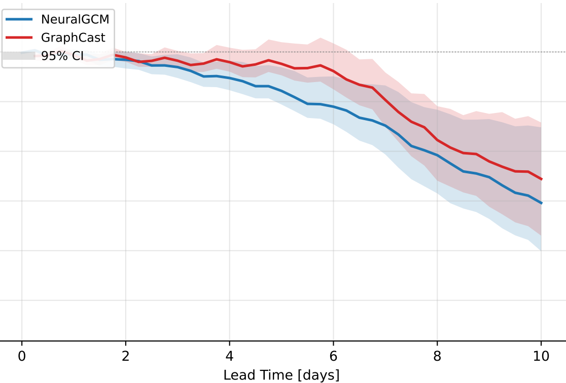
temperature@850 hPa — mean bias over all mixture heat waves (16 events, > p99)
