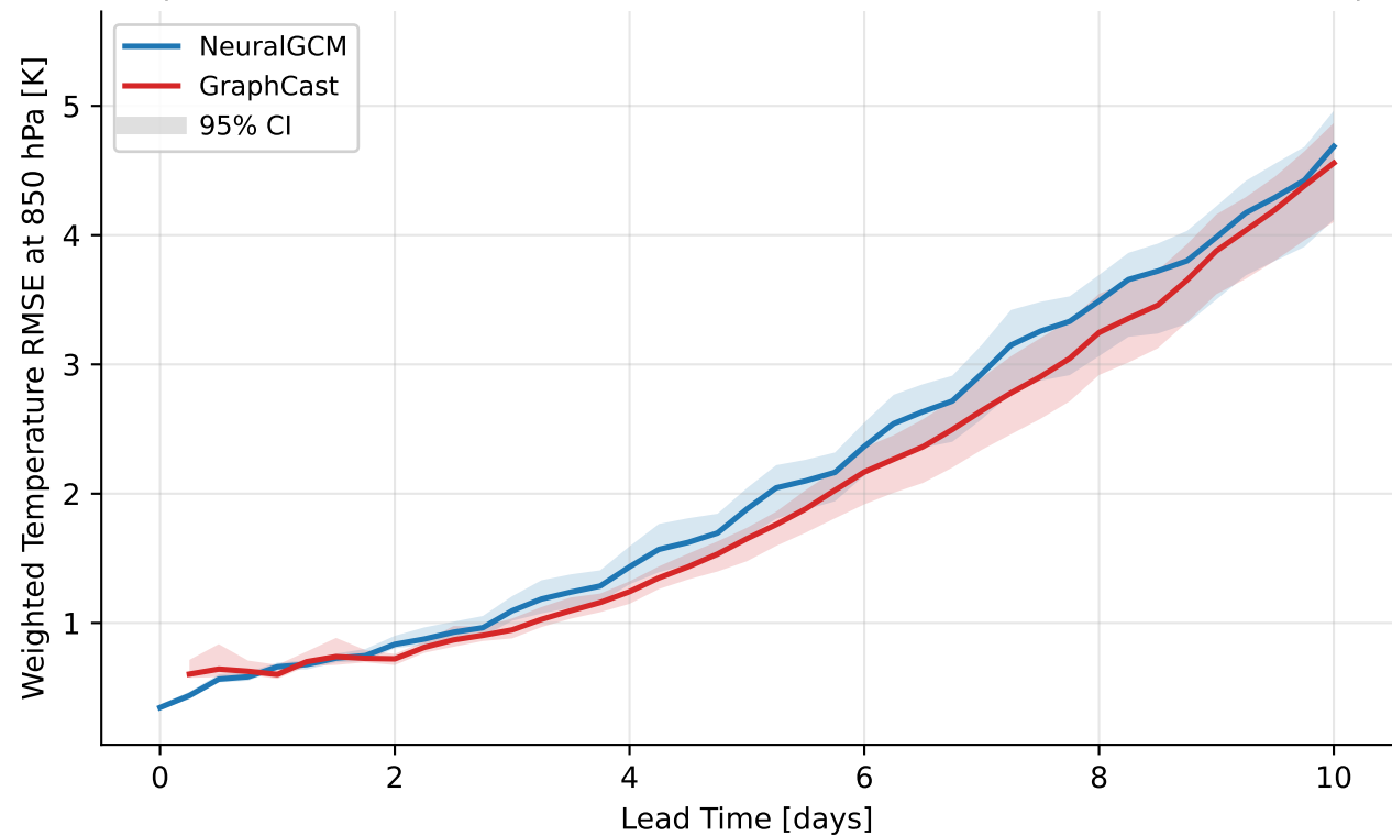
temperature@850 hPa — mean RMSE over all mixture heat waves (16 events, > p99)
