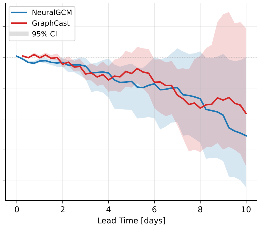
geopotential@500 hPa — mean bias over mixture heat waves per year (> p99)
