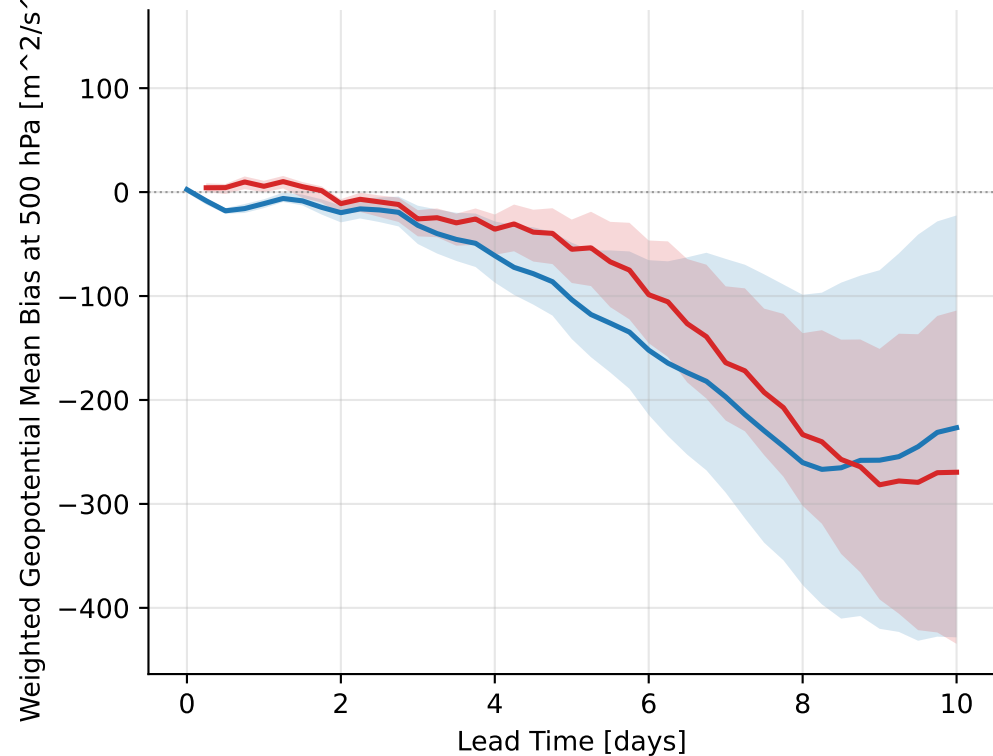
geopotential@500 hPa — mean bias over mixture heat waves per year (> p99)
