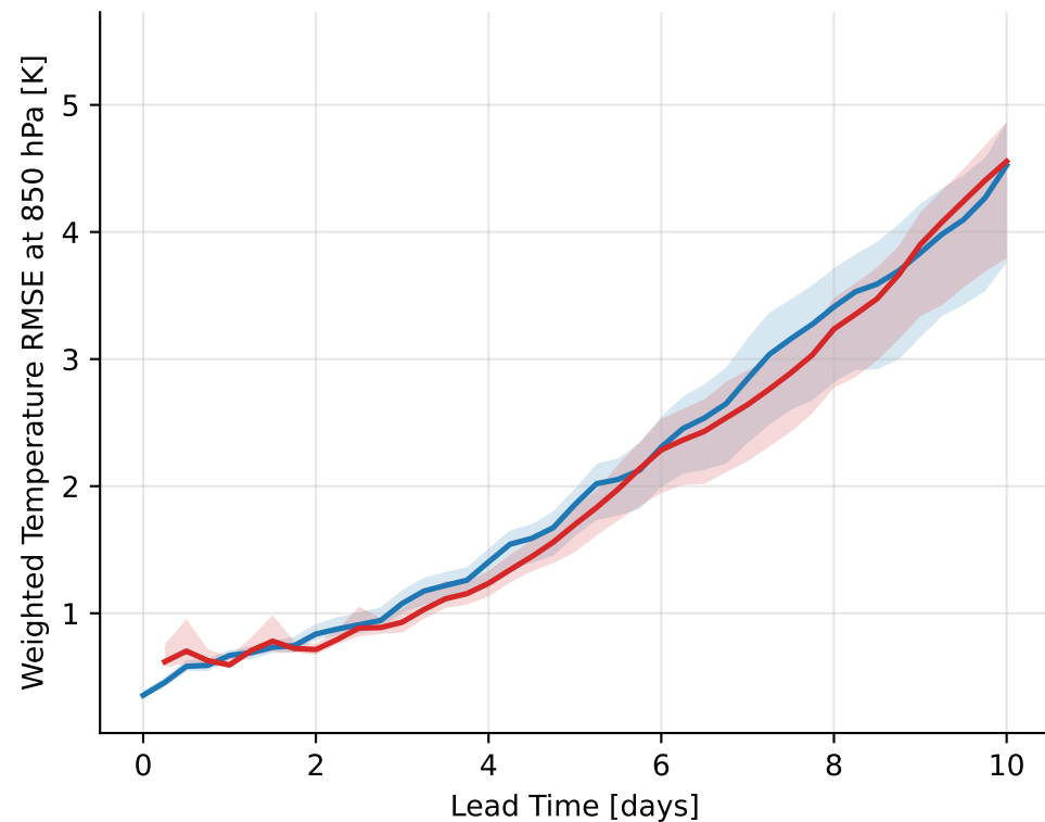
temperature@850 hPa — mean RMSE over mixture heat waves per year (> p99)
