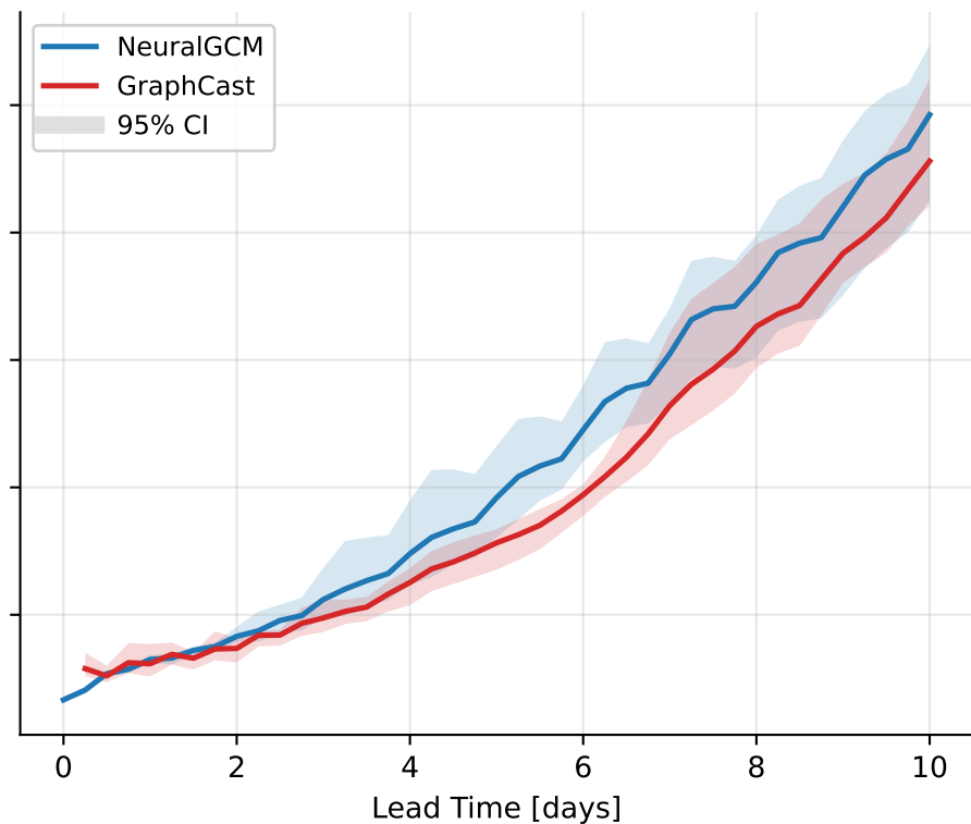
temperature@850 hPa — mean RMSE over mixture heat waves per year (> p99)
