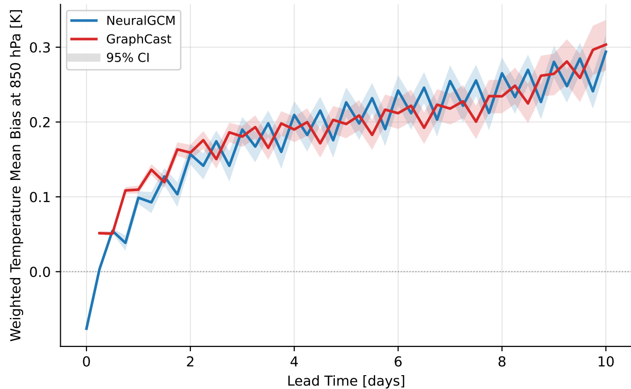
NeuralGCM vs GraphCast — 2049, 850 hPa temperature (global, mean of 355 inits)
