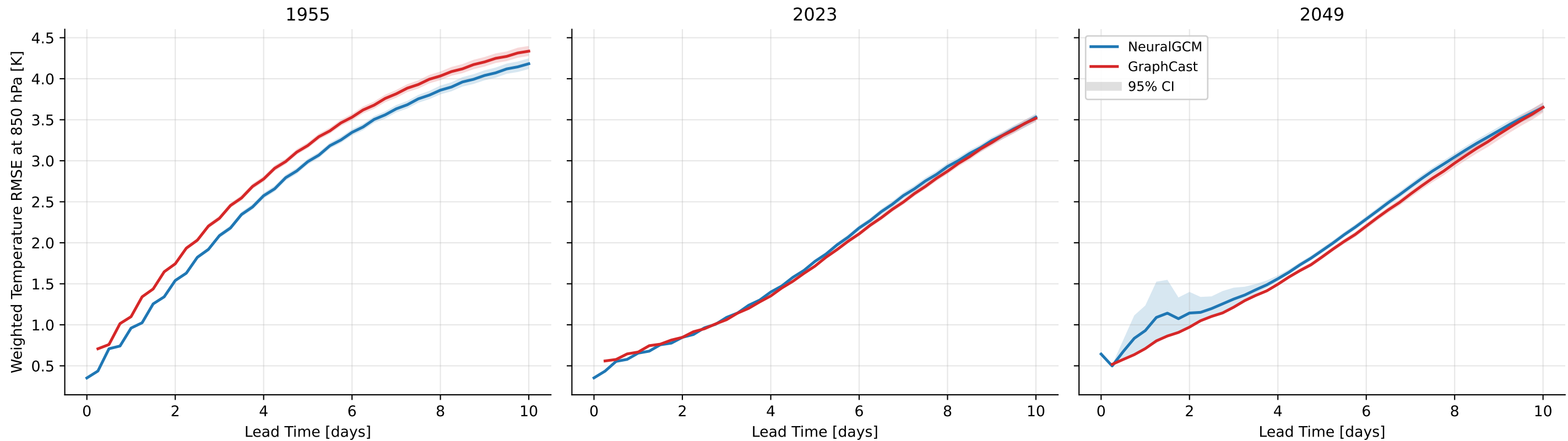
NeuralGCM vs GraphCast — temperature@850 hPa (global)
