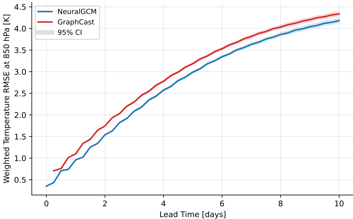
NeuralGCM vs GraphCast — 1955, 850 hPa temperature (global, mean of 355 inits)
