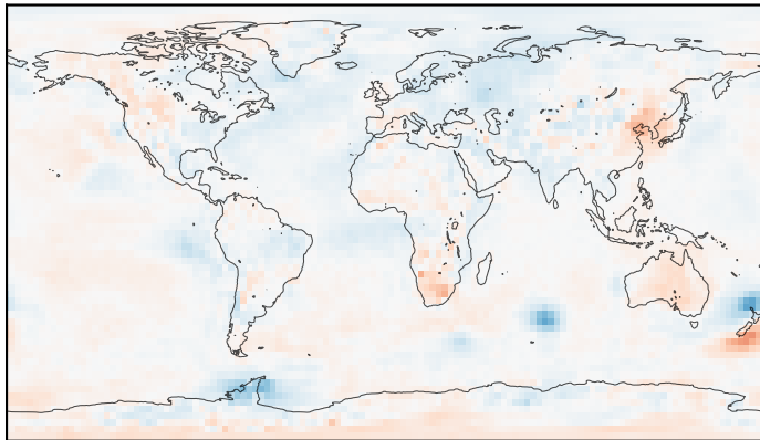
NeuralGCM
