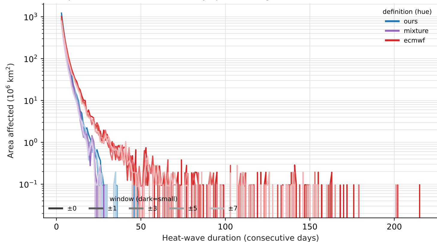
2023 heat waves by definition & window — area 95th-ptile, 1991-2020 ref, \geq 3 -day spells, 2.8^\circ grid
