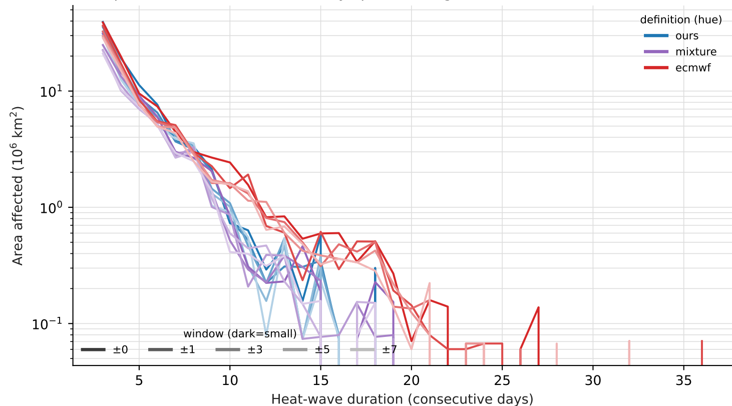
Europe — 2023 heat waves by definition & window — area 95th-pctile, 1991-2020 ref, \geq 3 -day spells, 2.8^\circ grid
