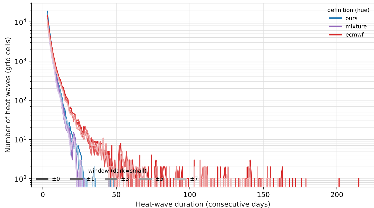
2023 heat waves by definition & window — count 95th-pctile, 1991-2020 ref, \geq 3 -day spells, 2.8^\circ grid
