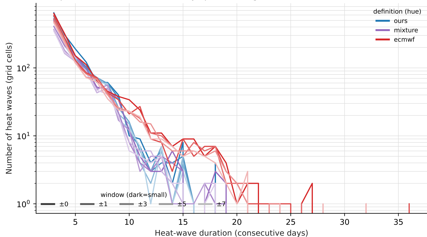
Europe — 2023 heat waves by definition & window — count 95th-pctile, 1991-2020 ref, \geq 3 -day spells, 2.8^\circ grid
