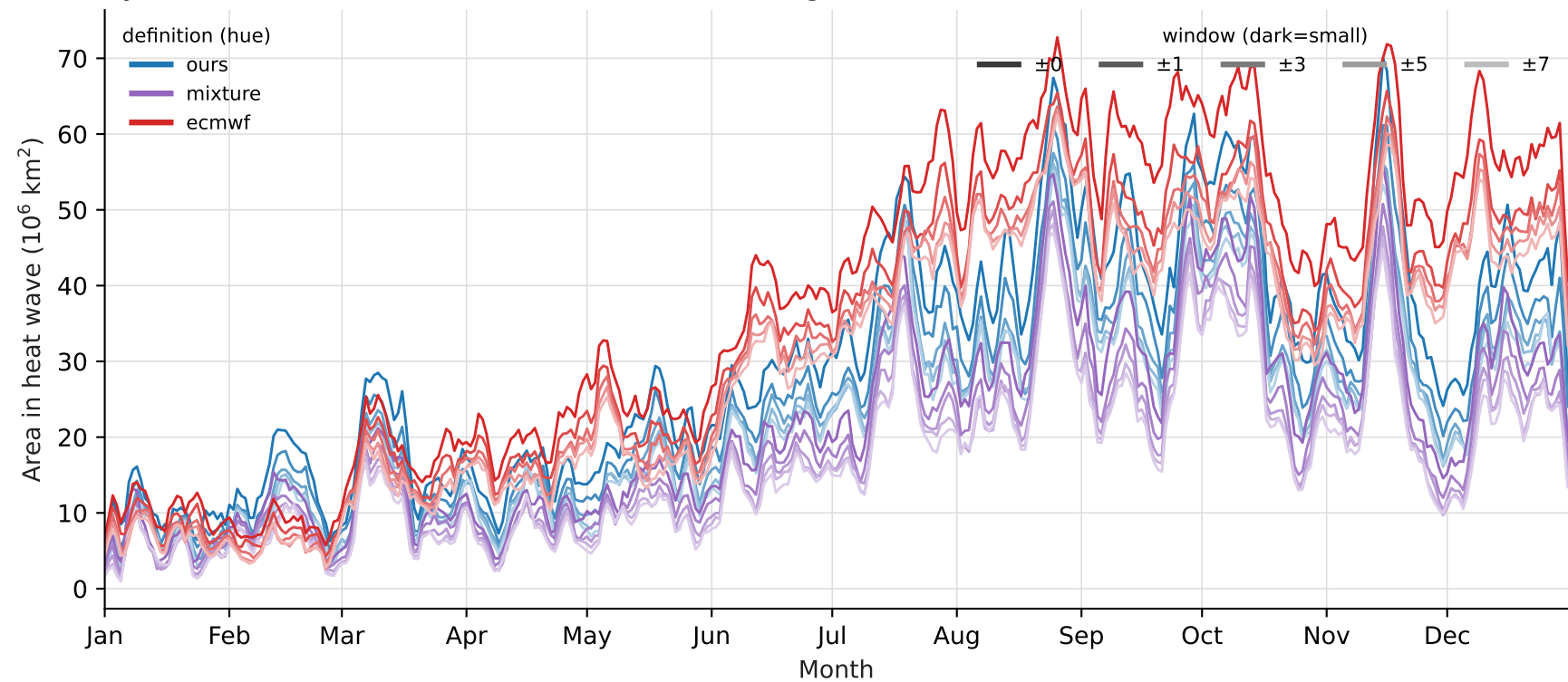
2023 — when heat waves occur (area in heat wave per day) by definition (hue) & \pm window (dark=small), 2.8° grid
