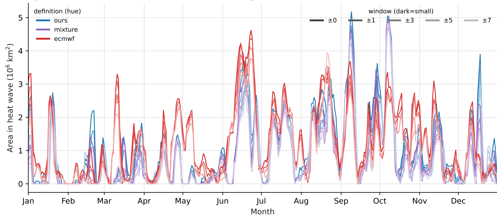
Europe — 2023 — when heat waves occur (area in heat wave per day) by definition (hue) & \pm window (dark=small), 2.8° grid
