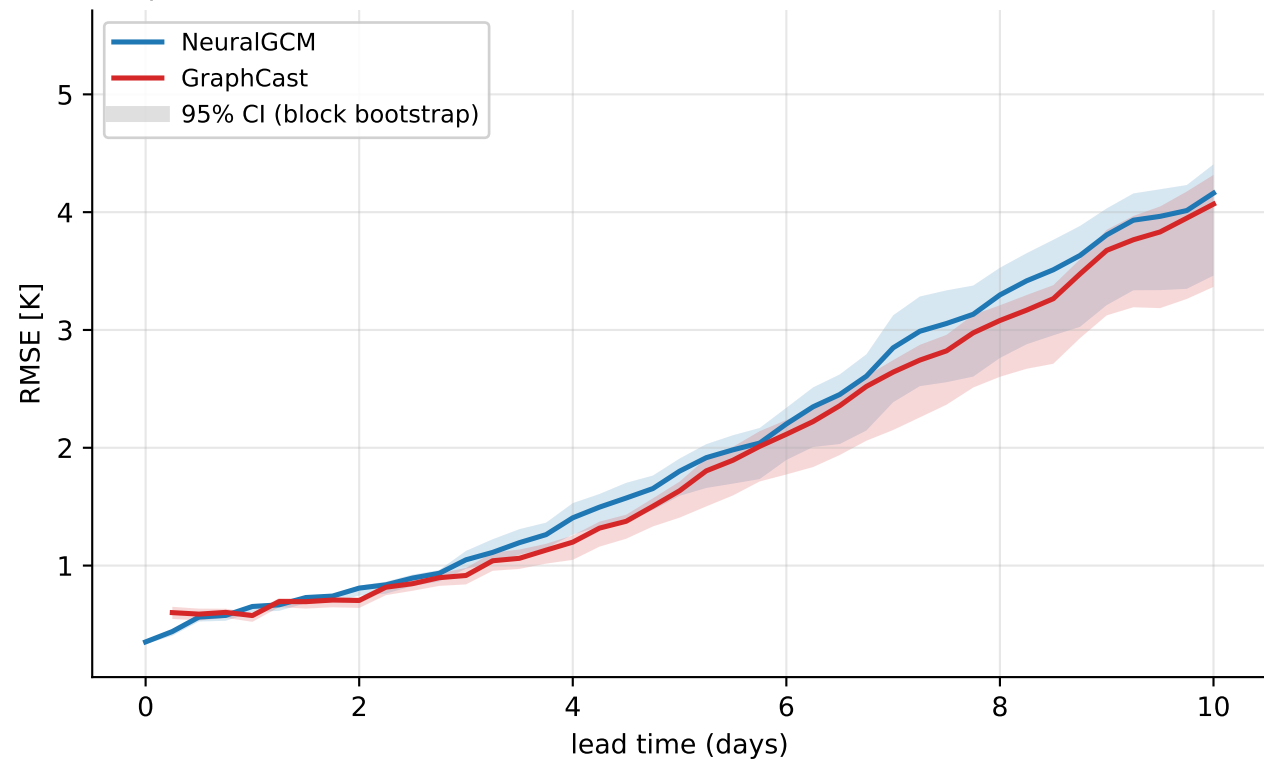
temperature@850 hPa — mean RMSE over the 6 2023 cordex heat waves (6 events, > p99)
