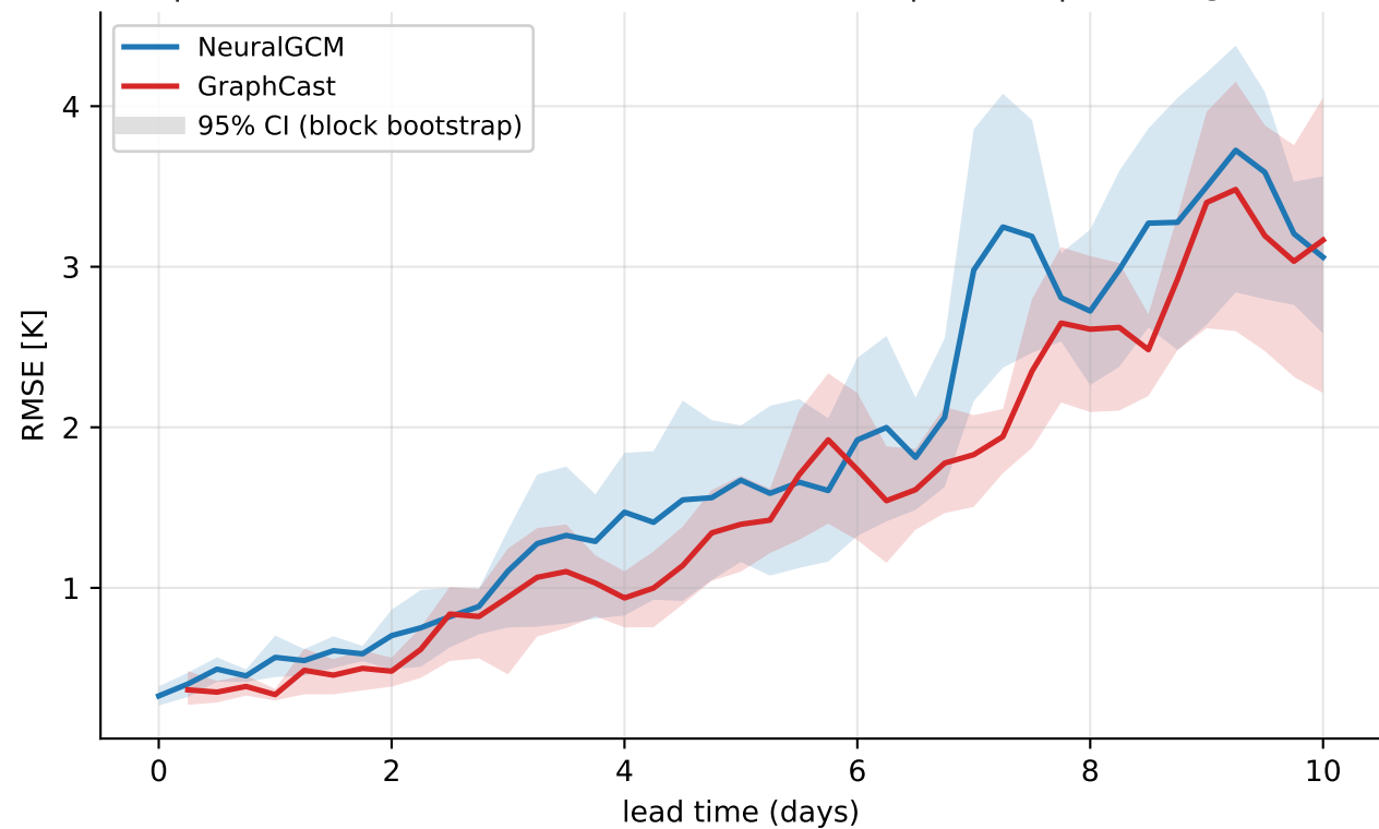
Europe heat-wave 2023-06-22..2023-06-25 — footprint temperature@850 hPa (mean of 14 rollouts)
