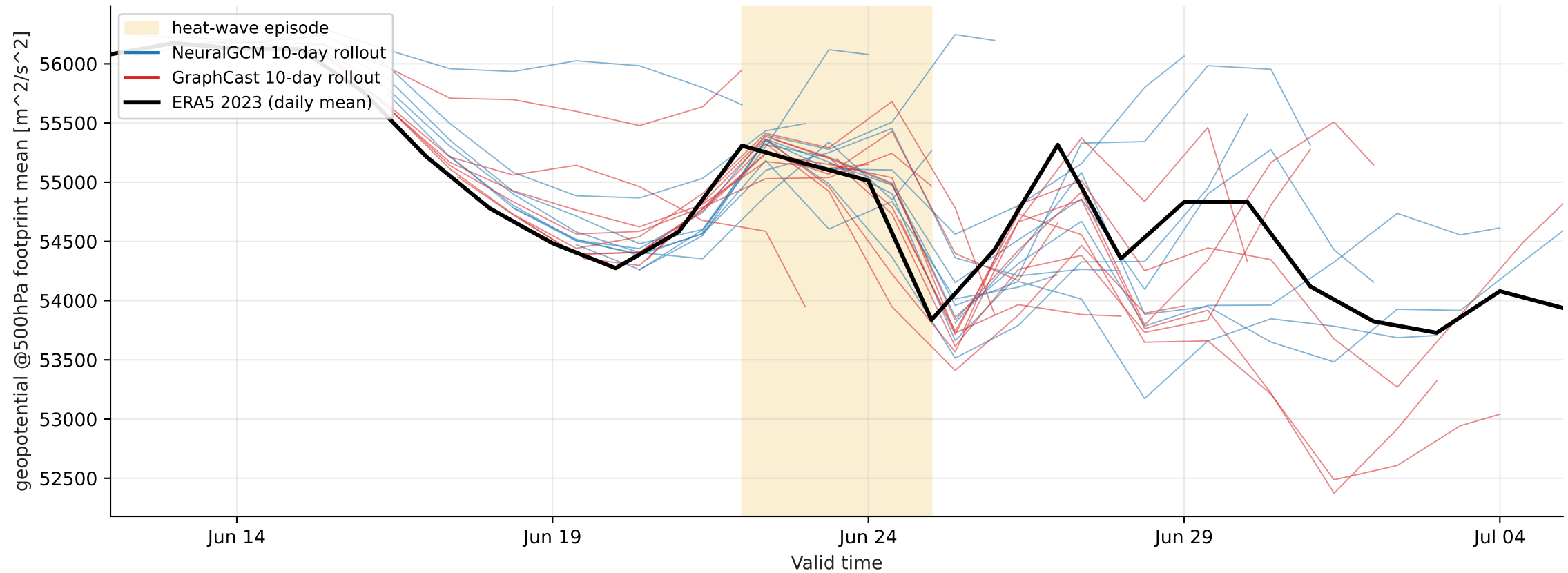
Europe heat-wave 2023-06-22..2023-06-25 — footprint-mean geopotential @ 500 hPa (cordex, > p99)
