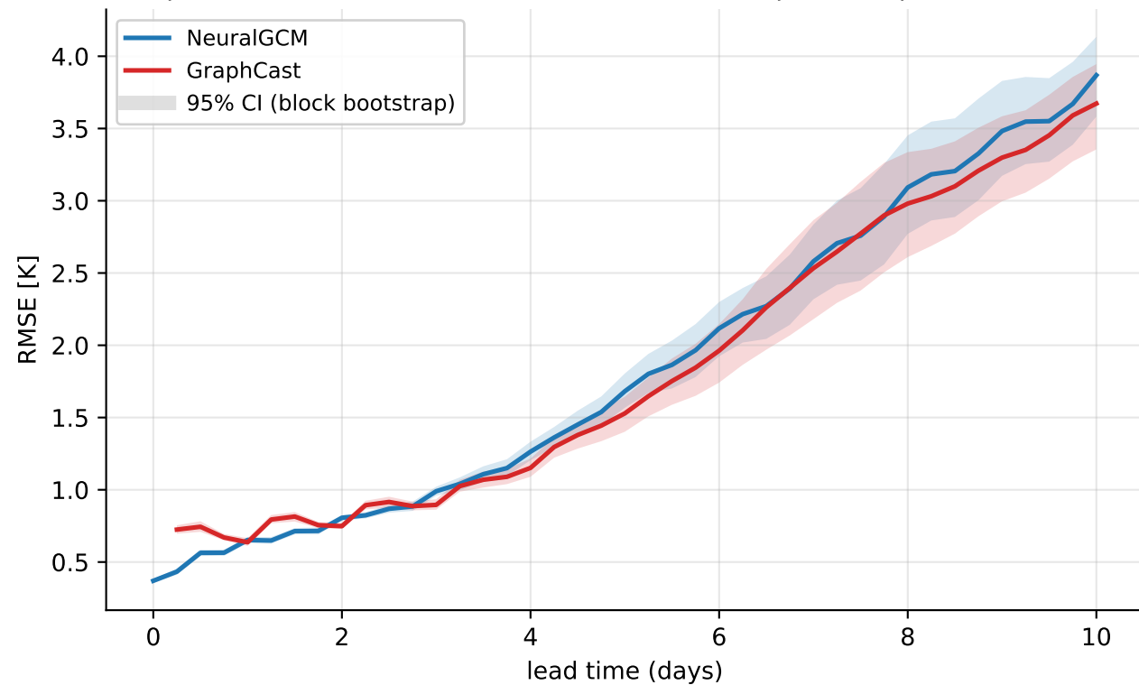
Europe heat-wave 2023-07-05..2023-09-01 — footprint temperature@850 hPa (mean of 69 rollouts)
