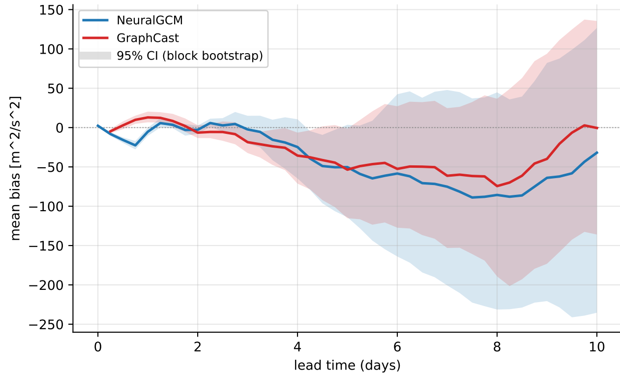
Europe heat-wave 2023-08-06..2023-09-12 — footprint geopotential@500 hPa (mean of 48 rollouts)
