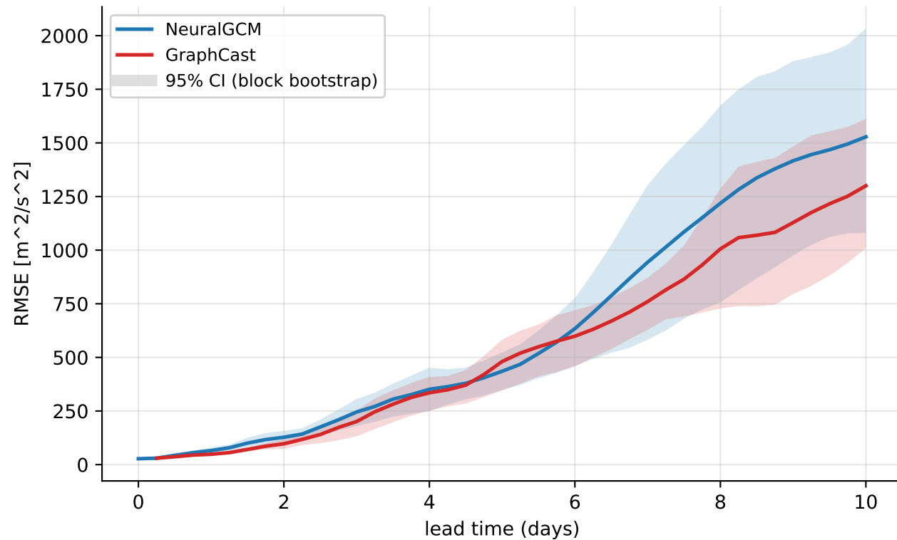
Europe heat-wave 2023-08-09..2023-08-28 — footprint geopotential@500 hPa (mean of 30 rollouts)
