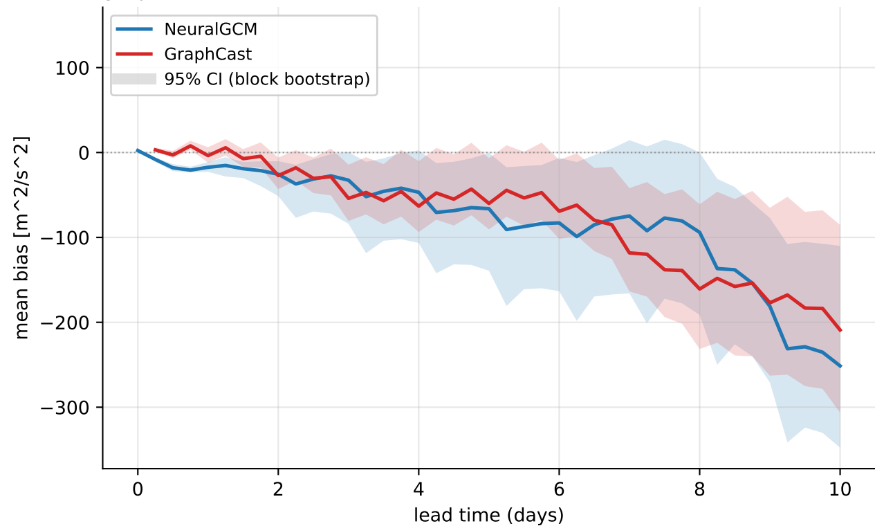
geopotential@500 hPa — mean bias over the 3 2026 cordex heat waves (3 events, > p99)
