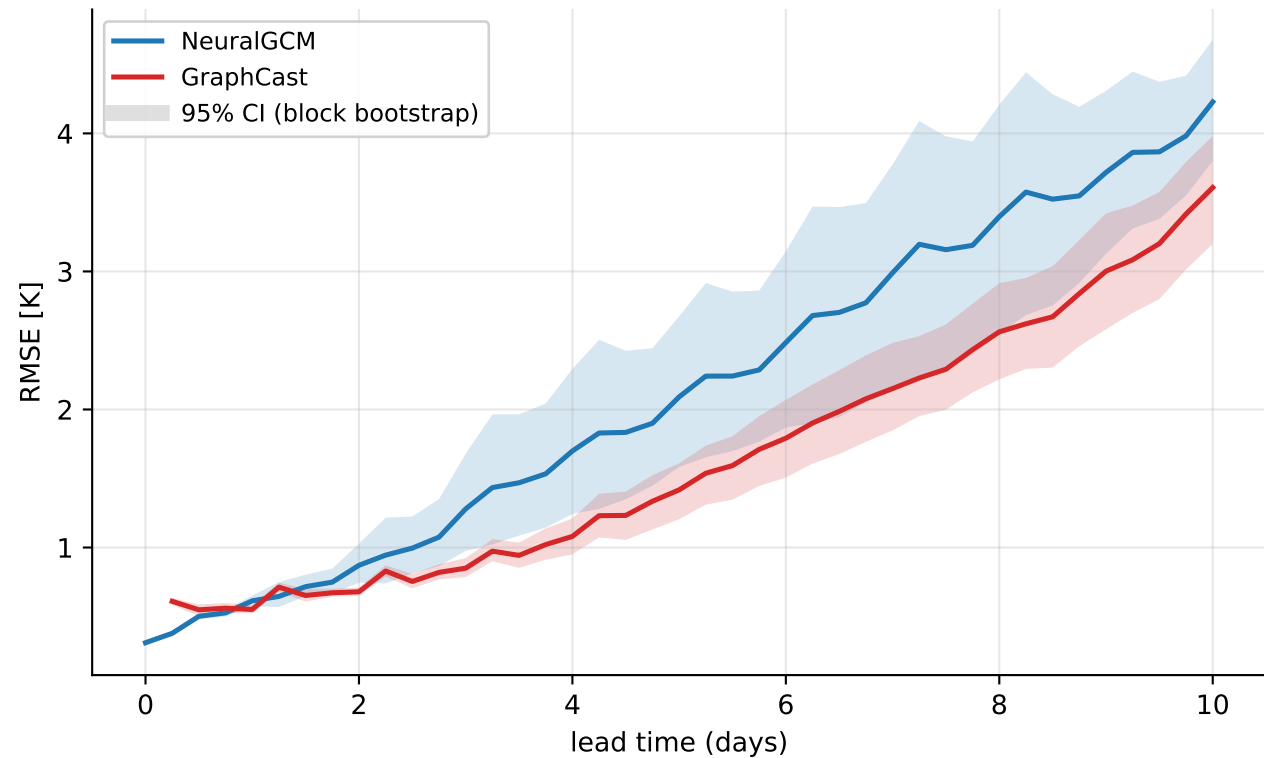
Europe heat-wave 2026-06-17..2026-07-24 — footprint temperature@850 hPa (mean of 36 rollouts)
