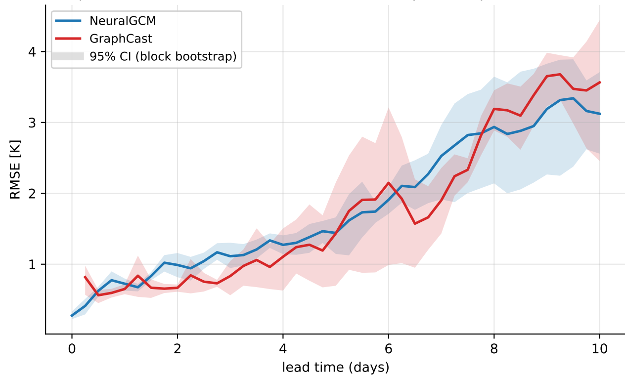
Europe heat-wave 2023-04-25..2023-04-28 — footprint temperature@850 hPa (mean of 14 rollouts)
