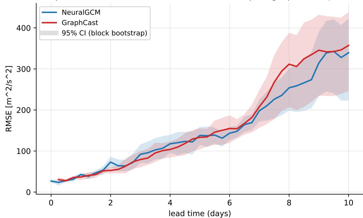
Europe heat-wave 2023-08-08..2023-08-19 — footprint geopotential@500 hPa (mean of 22 rollouts)
