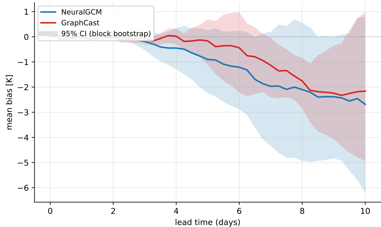
Europe heat-wave 2023-09-03..2023-09-09 — footprint temperature@850 hPa (mean of 17 rollouts)
