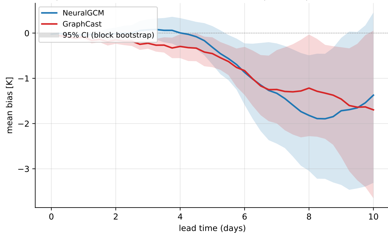
Europe heat-wave 2023-09-29..2023-10-11 — footprint temperature@850 hPa (mean of 23 rollouts)
