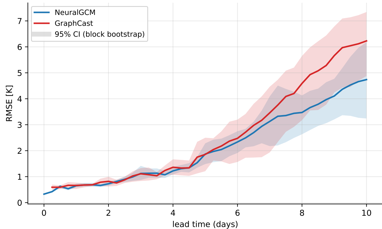
Europe heat-wave 2023-10-06..2023-10-11 — footprint temperature@850 hPa (mean of 16 rollouts)
