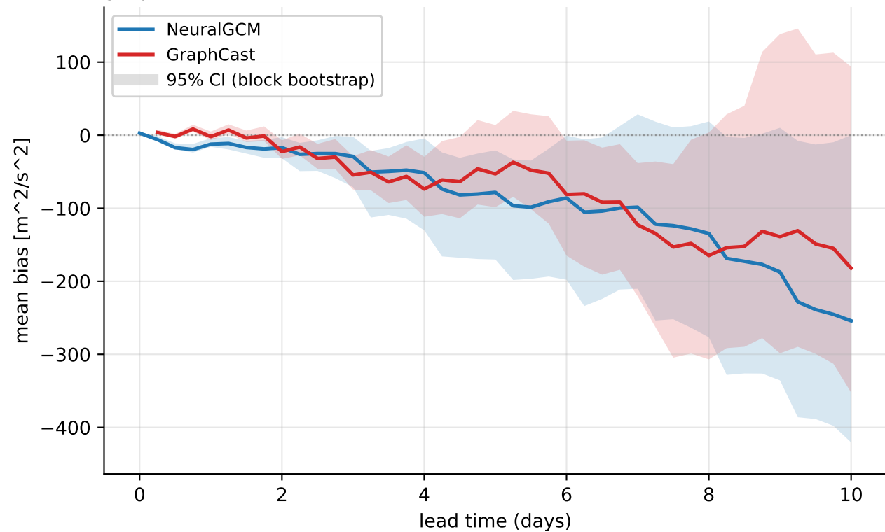
geopotential@500 hPa — mean bias over the 6 2026 mixture heat waves (6 events, > p99)
