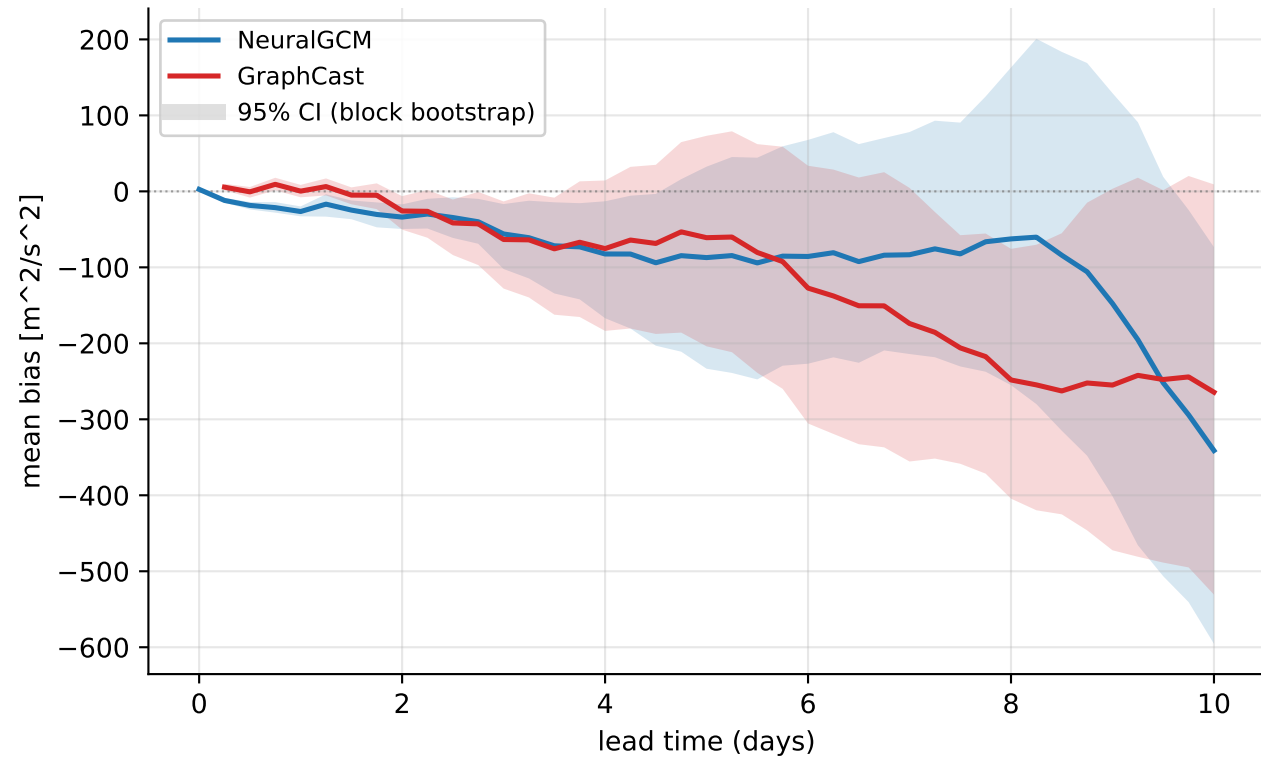
Europe heat-wave 2026-06-21..2026-07-01 — footprint geopotential@500 hPa (mean of 21 rollouts)
