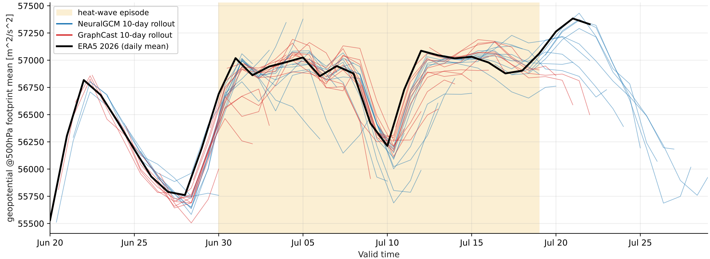
Europe heat-wave 2026-06-30..2026-07-19 — footprint-mean geopotential @ 500 hPa (mixture, > p99)
