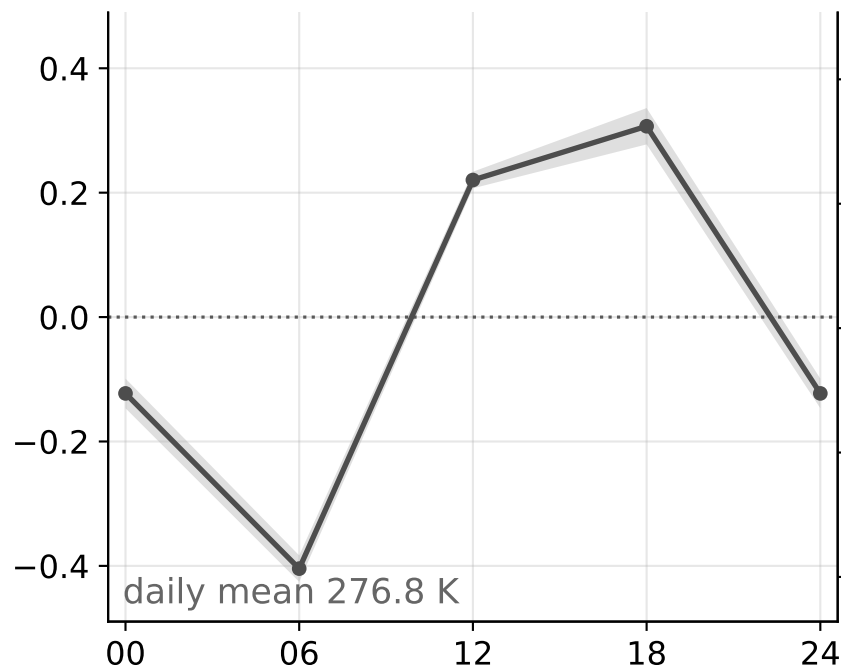
Temperature @ 850 hPa offset from daily mean [K]
