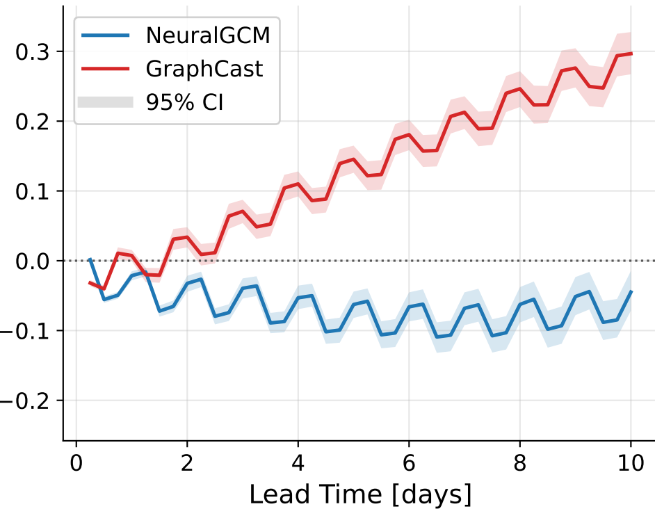
Weighted Temperature Mean Bias at 850 hPa
