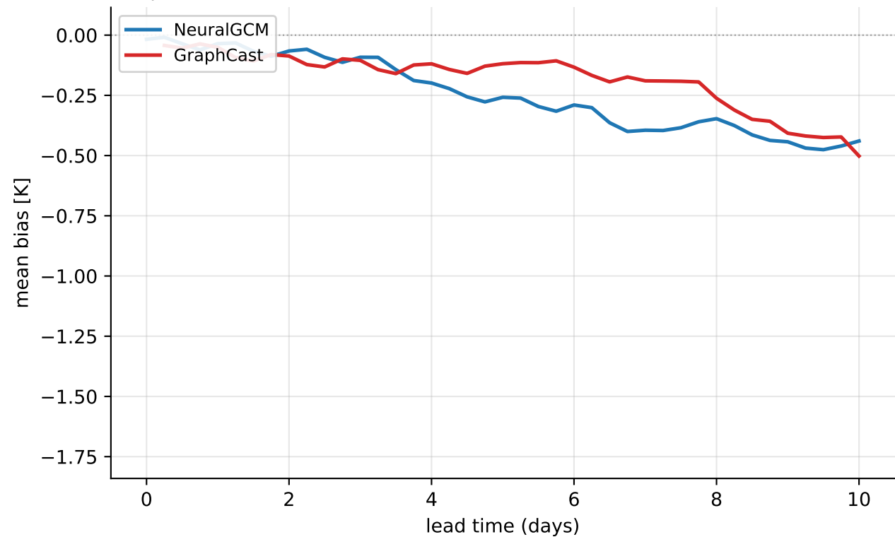
temperature@850 hPa — mean bias over the 6 2023 cordex heat waves (6 events, > p99)
