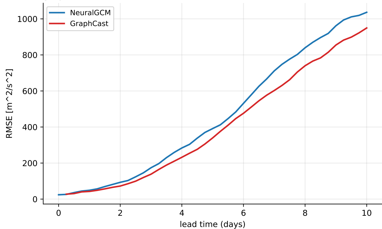
geopotential@500 hPa — mean RMSE over the 6 2023 cordex heat waves (6 events, > p99)
