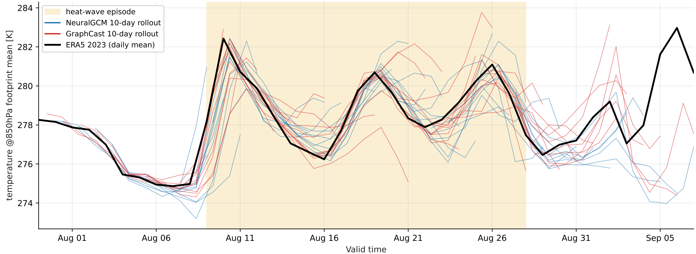
Europe heat-wave 2023-08-09..2023-08-28 — footprint-mean temperature @ 850 hPa (cordex, > p99)
