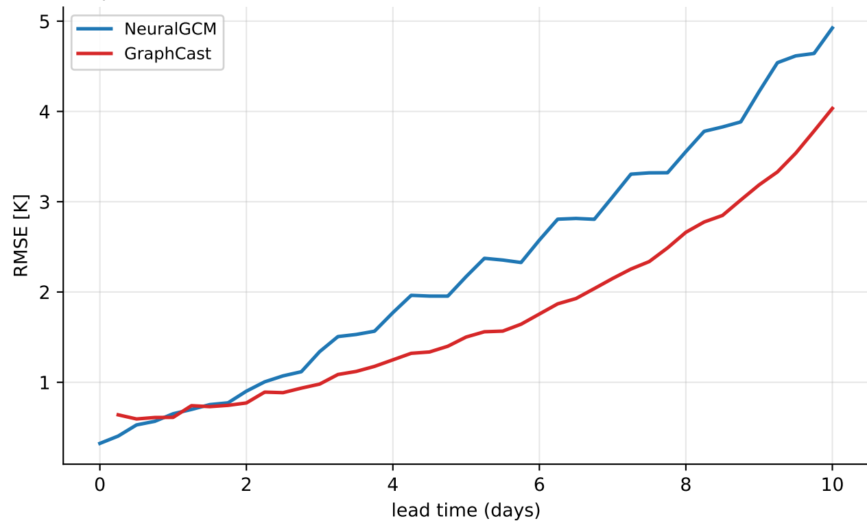
temperature@850 hPa — mean RMSE over the 3 2026 cordex heat waves (3 events, > p99)
