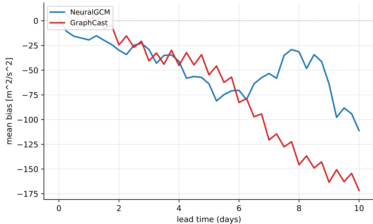
Europe heat-wave 2026-06-17..2026-07-24 — footprint geopotential@500 hPa (mean of 36 rollouts)
